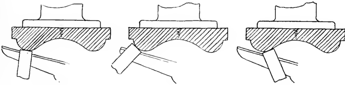
FIG. 322. CONVEX SCRAPING WITH SQUARE NOSE SCRAPER.
